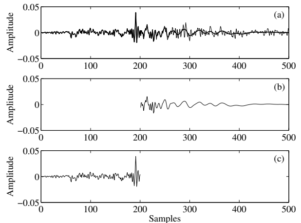
Fig. 9: Time-domain responses of the parallel filter used in Fig. 8: (a) target impulse response (thin line) and filter response (thick line), (b) the response of the second-order sections, and (c) the response of the 200th order FIR part.
