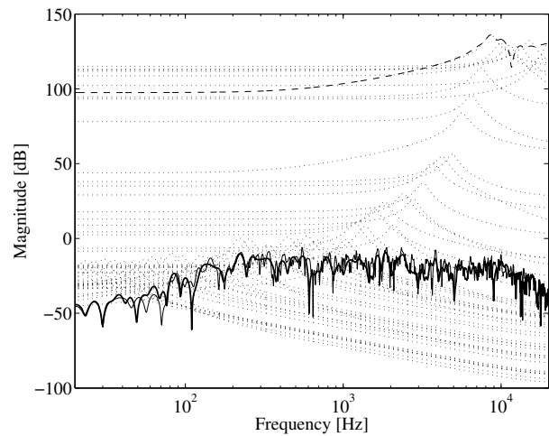
Fig. 6: Fixed-pole parallel filter design based on a piano soundboard response. Thin line: target frequency response, thick line: filter response, dashed line: frequency response of the FIR part, dotted lines: the individual responses of the second-order sections.
