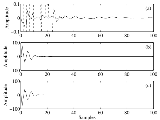
Fig. 2: Time-domain responses of the parallel filter used in Fig. 1: (a) filter impulse response (solid line) and the summed impulse response of the second-order sections (dashed line, clipping), (b) the response of the second-order sections in a different scale, and (c) the response of the 30th order FIR part.
