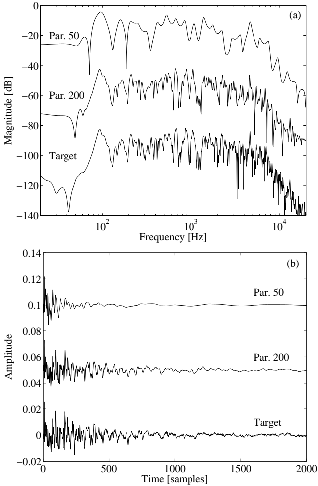
Figure 4. Frequency (a) and time-domain (b) responses of parallel second-order sections designed with logarithmic pole positioning for orders of 50 (top) and 200 (middle), and the target impulse response (bottom).
