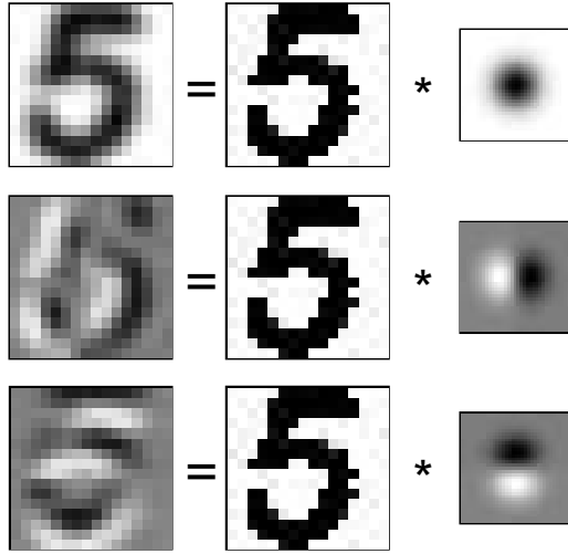
Fig. 12.12. Graphic illustration of the computation of f and two tangent vectors corresponding to L_x = \partial/\partial x (X-translation) and L_y = \partial/\partial y (Y-translation), from a binary image I . The Gaussian function g(x, y) = \exp(-\frac{x^2+y^2}{2\sigma^2}) has a standard deviation of \sigma = 0.9 in this example although its graphic representation (small images on the right) have been rescaled for clarity.
