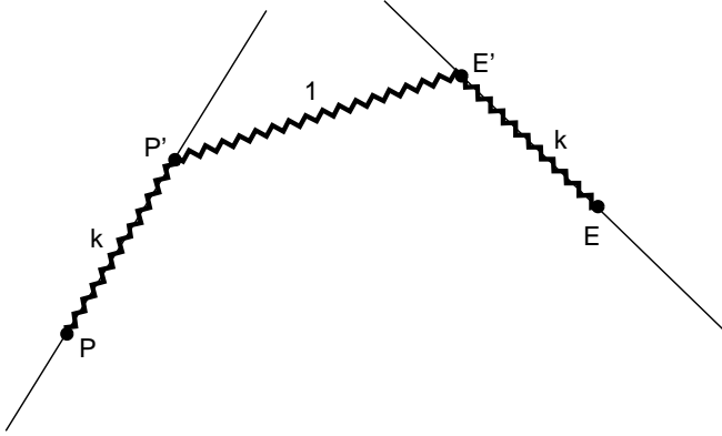
Fig. 12.7. The tangent distance between E and P is the elastic energy stored in each of the three springs connecting P, P', E' and E . P' and E' can move without friction along the tangent planes. The spring constants are indicated on the figure.
