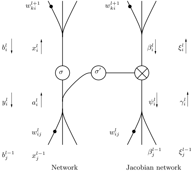
Fig. 12.9. Forward propagated variables (a, x, \gamma, \xi) , and backward propagated variables (b, y, \beta, \psi) in the regular network (roman symbols) and the Jacobian (linearized) network (greek symbols). Converging forks (in the direction in which the signal is traveling) are sums, diverging forks just duplicate the values.
