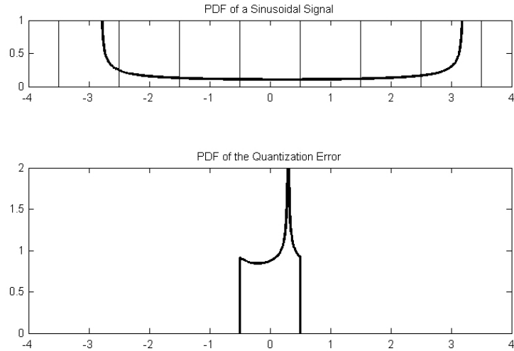
Fig. 2 Probability density function of a sinusoidal signal (amplitude: 3), and that of the quantization error. The dc offset is dc = 0.2 .
