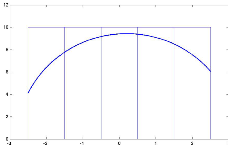
Fig. 5 Weighting by the reciprocal of the probability density function
