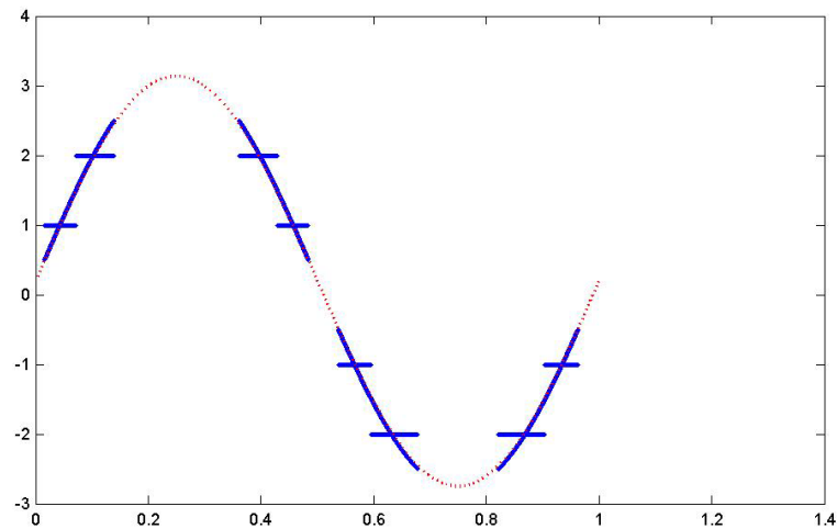
Fig. 6 Improved fitting of the samples of a quantized sine wave with weighting by the reciprocal of the PDF of the sine wave, and eliminating the samples in the central bin
