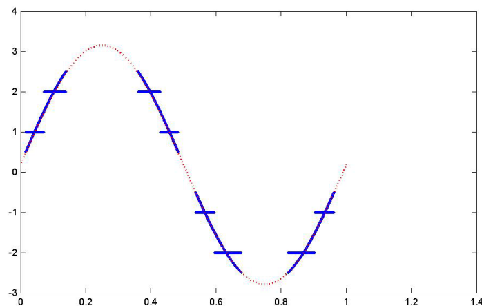
Fig. 8 Improved fitting the samples of a quantized sine wave with weighting by the reciprocal of the PDF of the sine wave, maintaining the probability in each bin, and eliminating the very small samples
