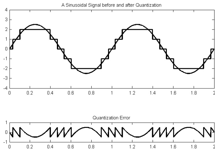
Fig. 1 Quantization of a sine wave in an ideal quantizer, with quantum size = 1, and dc offset 0
