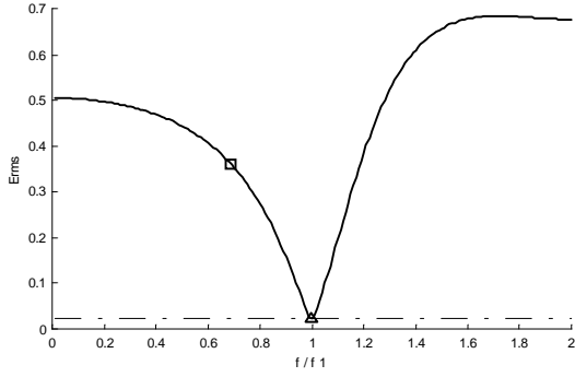
Fig. 1 – The rms error of the three parameter algorithm (in LSB) as a function of the applied frequency value (shown as related to the nominal value). f_j=0.020773f_s , M=70 points, no noise.
