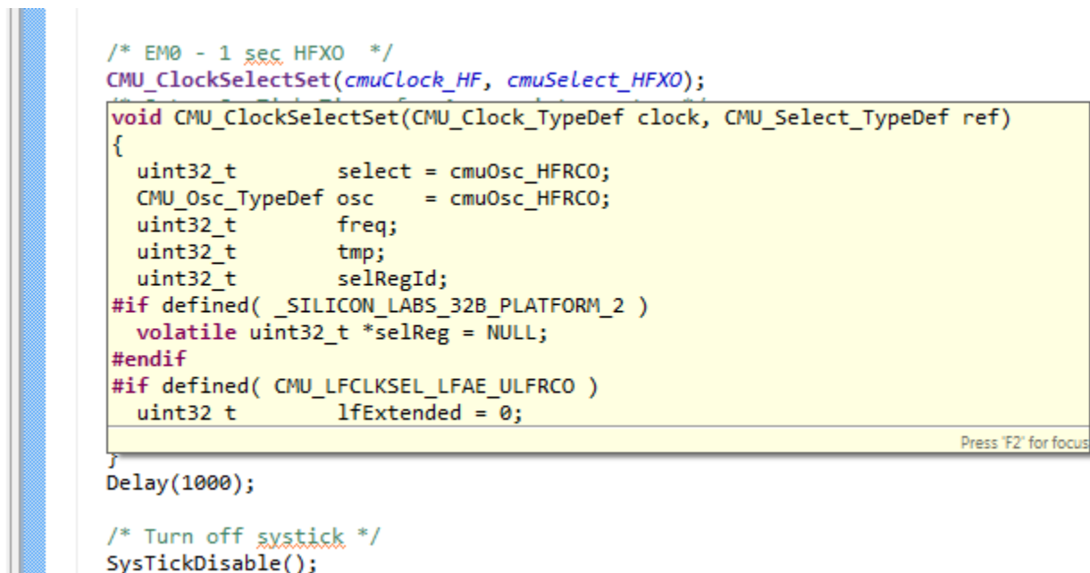
Figure 3.5. Symbol Expansion
