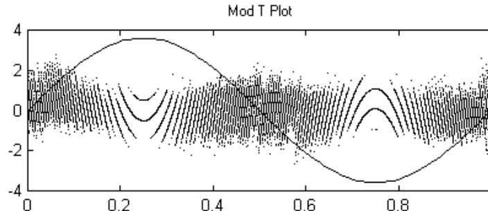
Figure 1: An example: the Modulo Time Plot [6]
