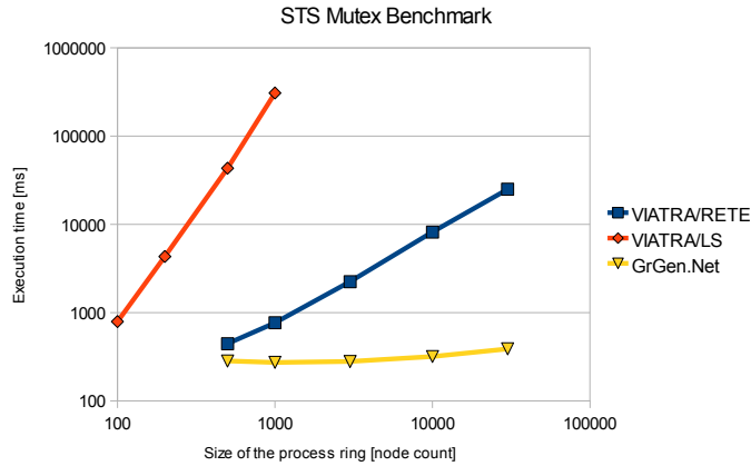
Fig. 12. Results for the STS mutex benchmark
