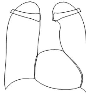
(i) b_3 = +3\sqrt{\lambda_3}
