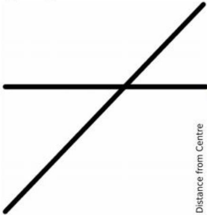
Input Image
