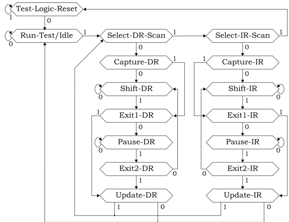
JTAG state machine (just for illustration purposes)
